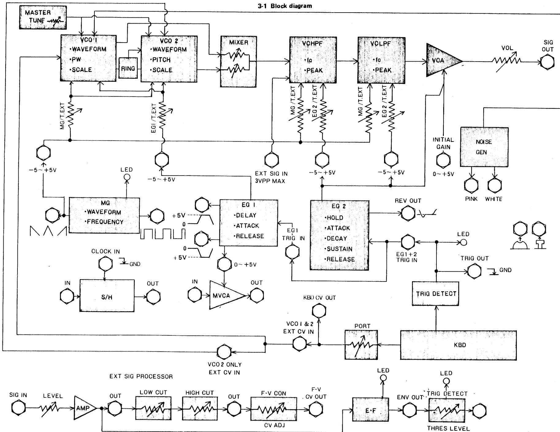
3-1 Block diagram
